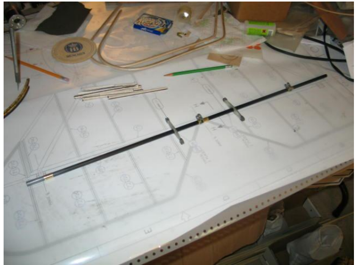
Brass tube, hinges, ctrl horns on carbon tube
