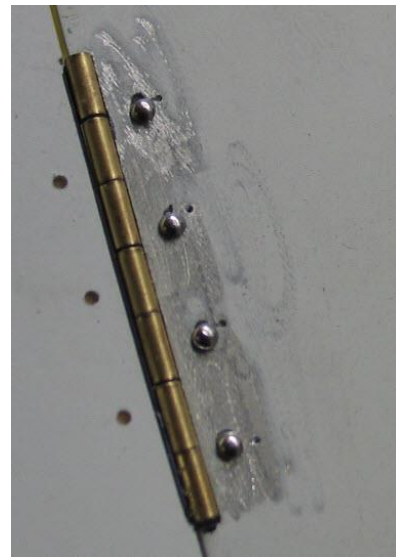
Close-up of door, hinge and panel
