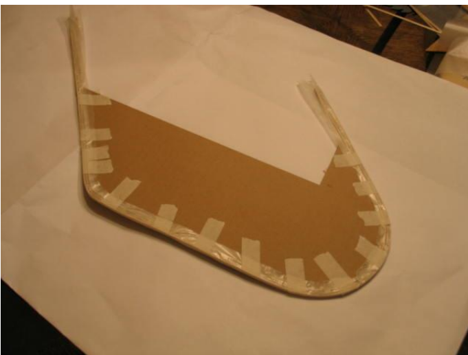
Laminated outline parts taped in place
