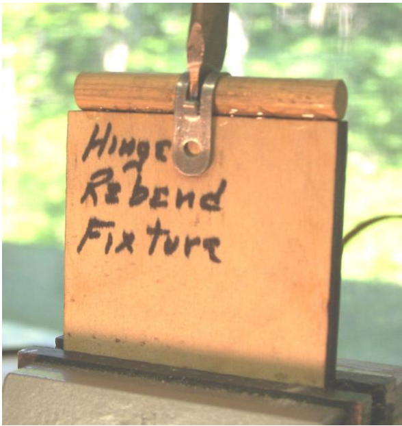
Screw driver used to bend hinge strap
