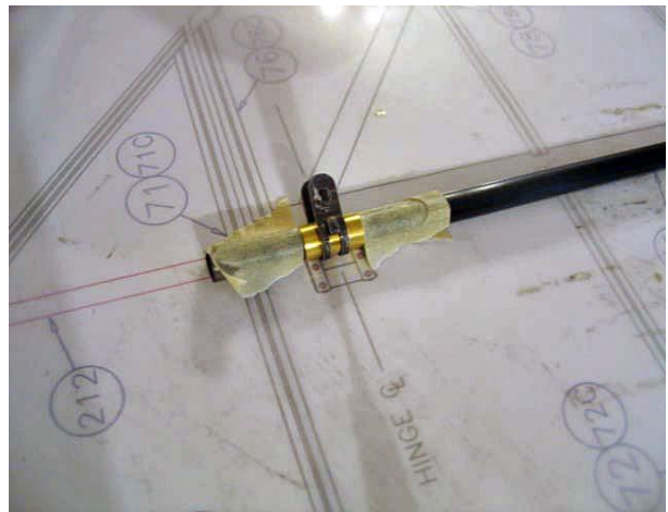
Tape hinge outside collars
