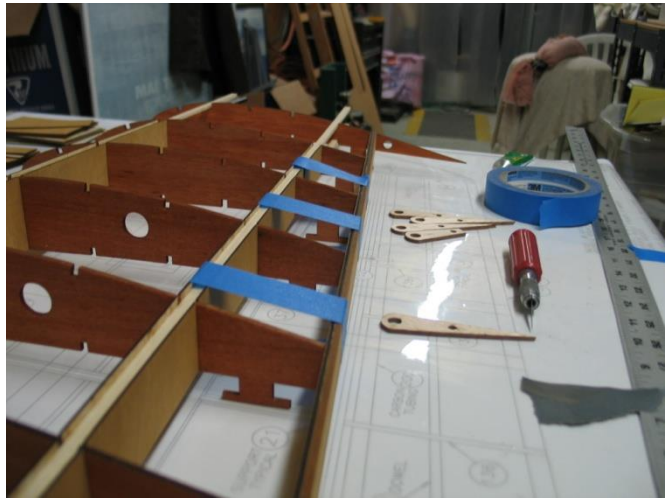
Ensure aileron leading edge is straight
