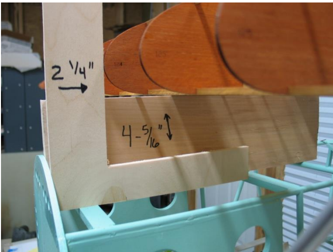
Locate wing using these dimensions
