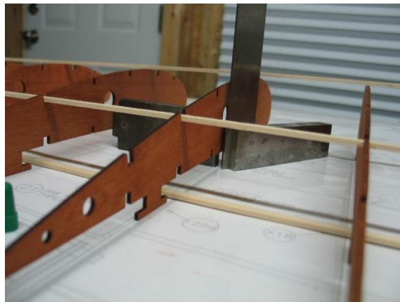
Use square to align ribs correctly
