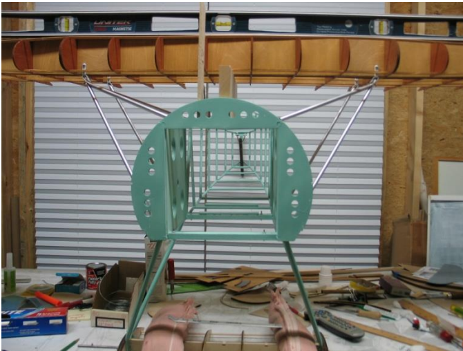
Use a level to keep wing level to fuselage
